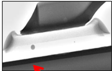
Solder ball
